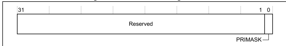
Figure 5. PRIMASK bit assignment
